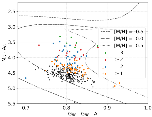
Figure 7. Showing the same data points as Figure 4 with indicated definite triple (green dots), possible triple (red dots), binary (blue dots), and possible binary stellar systems (orange dots). All other classes are shown with black dots. Overplotted are PARSEC isochrones (Marigo et al. 2017) for stars with the age of 4.5 Gyr and different metallicities.
