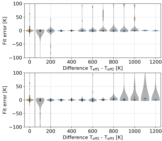
Figure 15. The accuracy of our analysis when the fitting procedure is applied to a synthetic triple system. Upper panel shows the distribution of T_{\text{eff}} prediction errors for a secondary star depending on the difference between selected temperatures of a primary and a secondary star. The lower panel shows the same relation but for a tertiary star in comparison to a secondary. As a reference, the prediction error of a primary star is shown on the left side of both panels. Labels T_{\text{eff}1} , T_{\text{eff}2} , and T_{\text{eff}3} indicate decreasing effective temperatures of stars in a simulated system.
