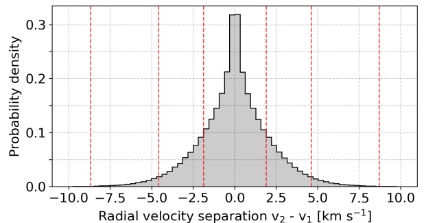
Figure 12. Same as Figure 10, but for an inner binary of a simulated triple stellar system.
