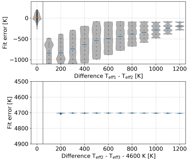
Figure B4. Similar to a plot in Figure 15, but representing a case when we try to describe a synthetic binary system with T_{\text{eff}3} = 0 using a triple star model.
