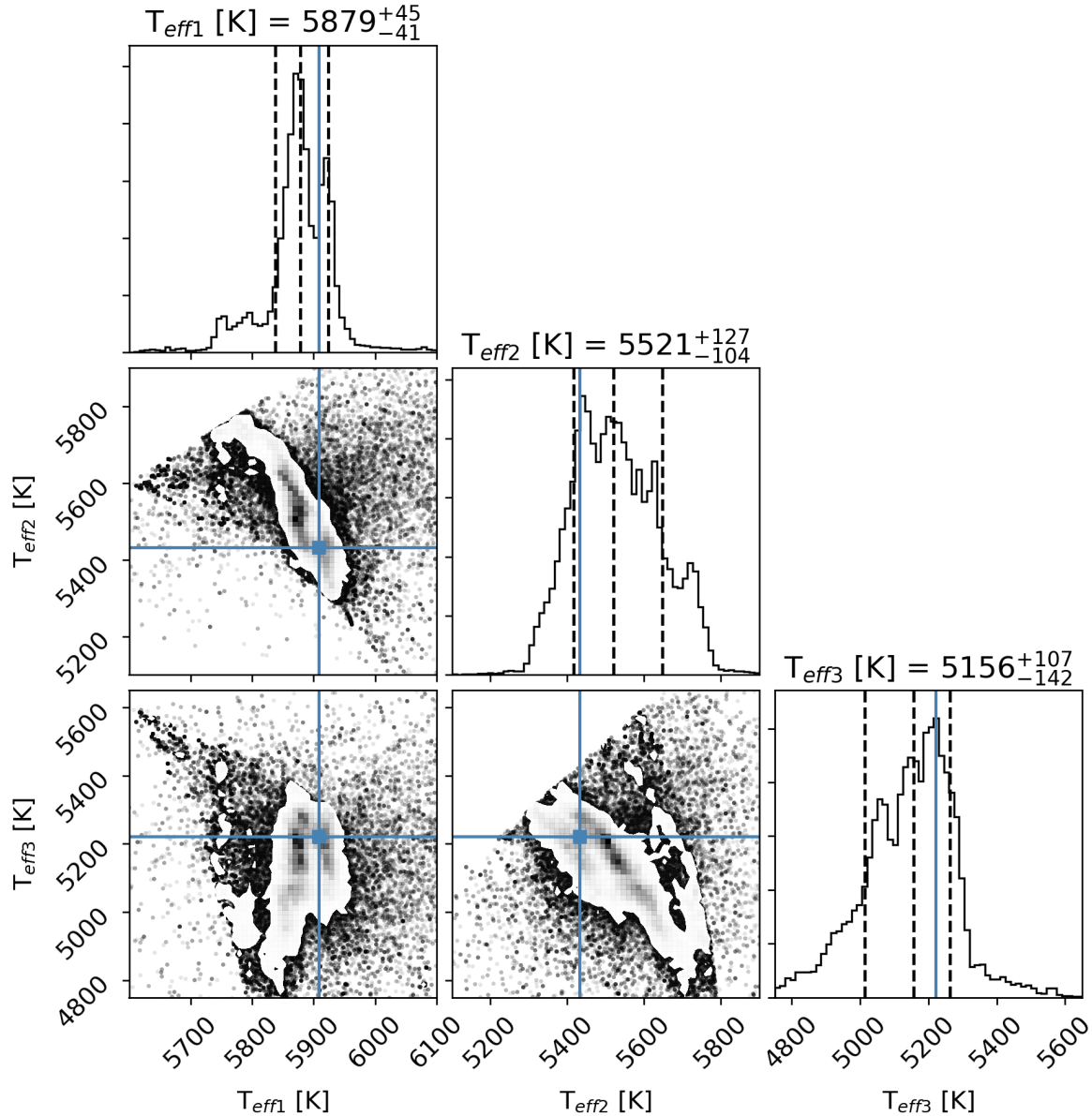
Figure 6. Distribution of considered posteriors during the initial MCMC photometric fit for one of the objects that was at the end classified as a triple candidate. As the plots show the first step in the fitting procedure that explores the complete parameter space, the distributions are not expected to be smooth because of possible multiple local minima. Values indicated on the scatter plots represent medians for the 10 % of the best fitting solutions.
