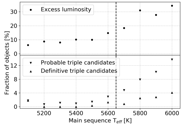
Figure 16. The upper panel shows the percentage of objects at different positions on the Kiel diagram shown in Figure 5 that show excessive luminosity and are spectroscopically similar to main sequence stars. Similarly, the lower panel shows upper and lower boundary on a percentage of triple system candidates at the same positions. For a definitive candidate, both fits must agree on a triple configuration. The strong dashed vertical line represents a point on Kiel diagram where the main sequence visually starts merging with the red-giant branch, the point where a region above the main sequence becomes polluted with more evolved stars.
