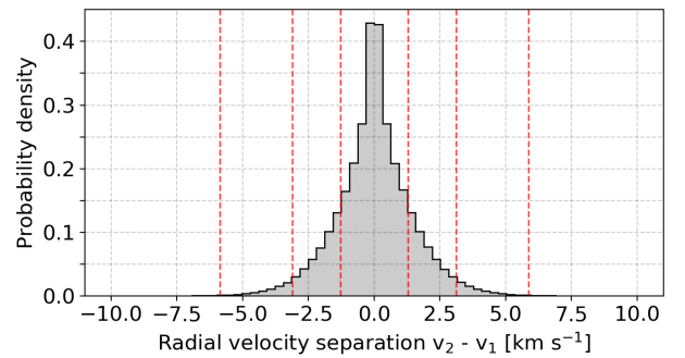
Figure 10. Distribution of computed radial velocity separations between a primary and secondary component of the simulated binary systems defined by the orbital parameters given in Table 4. Red vertical lines show 1, 2, and 3 \sigma probabilities of the given distribution.
