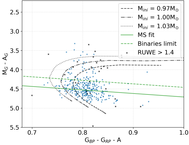
Figure 4. Gaia extinction corrected absolute G magnitude and colour index computed from G_{BP} , and G_{RP} bands. Stars marked with black crosses have large normalised astrometric uncertainty ( \text{RUWE} > 1.4 ). The green dashed line represents a threshold that was used as a delimiter between objects treated as multiple and single stars. Overlaid evolutionary tracks, constructed from the PARSEC isochrones (Marigo et al. 2017), represent an evolution of stars with Solar-like initial mass M_{ini} and metallicity [M/H] = 0 for stellar ages between 0.1 and 12 Gyr.
