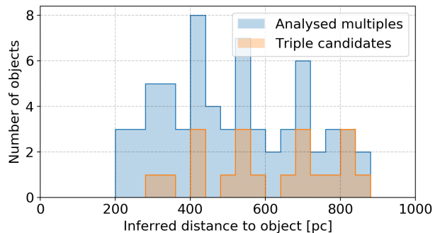
Figure 9. Histogram showing distribution of radial distances for the analysed set of stars. Distances were inferred by the Bayesian approach that takes into account the distribution of stars in the Galaxy (Bailer-Jones et al. 2018).
