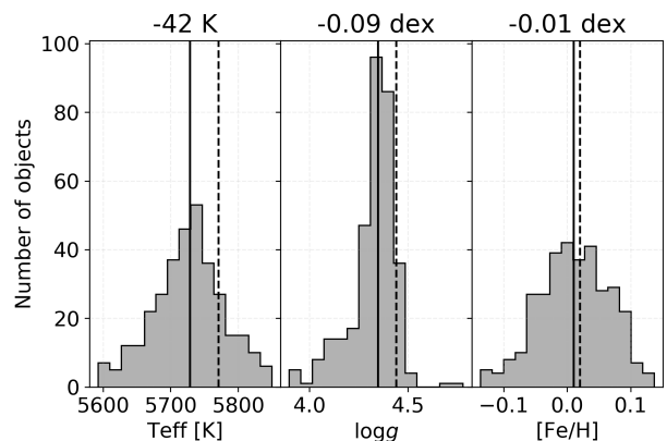
Figure 2. Distribution of physical parameters for discovered Solar twin candidates. Values above the plots represent difference between median of the distribution (solid vertical line) and actual Solar values (dashed vertical line).
