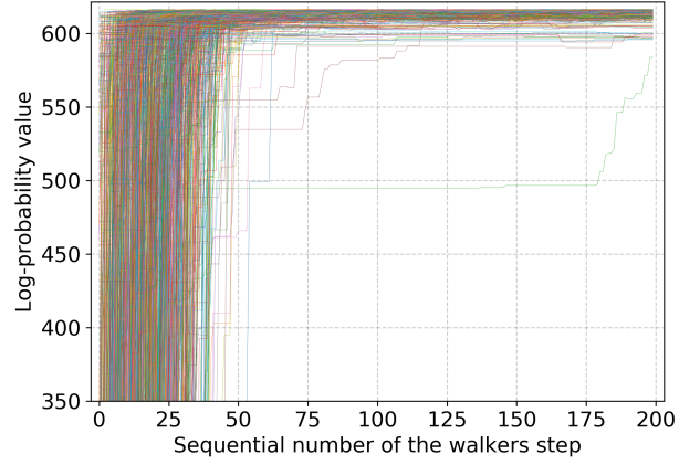
Figure B2. Convergence of walkers in the initial photometric fit. The plot shows a log-probability of the posteriors shown in the Figure 6. Walkers converge to the same value of log-probability after 50 steps. Every walker is plotted with different colour.
