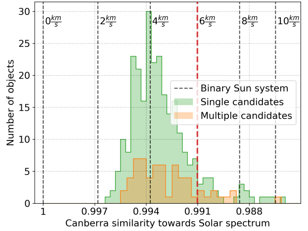
Figure B3. Same as Figure 14 but for the case of a triple system where only one component out of three has a radial velocity shift in comparison to other two.
