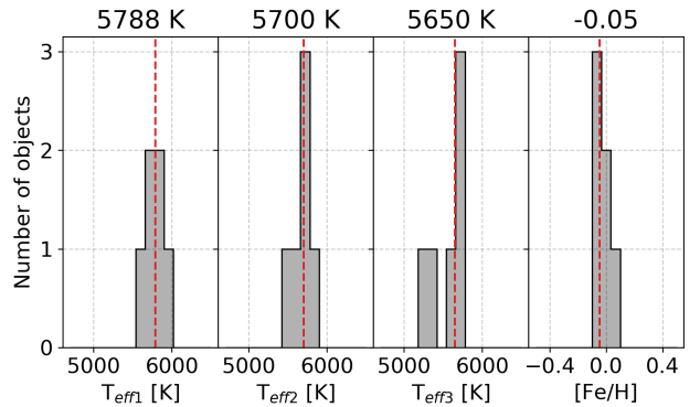
Figure 8. Parameters of triple stellar systems discovered and characterized by our analysis. Histograms represent distribution of all fitted results for 6 objects that were classified as triple stellar systems and observationally mimic Solar spectrum. Median values of the distributions are given above individual histogram and indicated with dashed vertical line.
