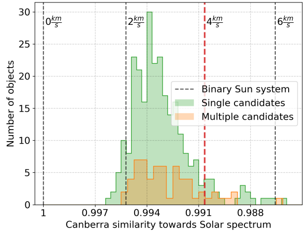
Figure 14. Histograms of Canberra similarities towards Solar spectrum for multiple stellar candidates (orange histogram) and single star candidates (green histogram) in the red HERMES arm. Vertical dashed lines represent the same similarity measure, but for a binary system comprising of two equally bright Suns, whose components are at different radial velocities. The separation between components is increasing in 2 \text{ km s}^{-1} steps, where the left-most vertical line represents the case where both stars are moving with the same projected velocity. The selected maximal velocity at which the composite spectrum would still be considered a Solar twin is marked with the thicker red vertical line. Distribution of histograms also shows that spectra of multiple system candidates are as (dis)similar as spectra of single stars.
